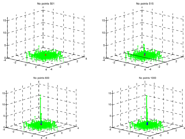
Fig. 13. The result of incremental LOF algorithm ( k=10 ) on dataset consisting of 500 records gaussian distribution N(\boldsymbol{\mu}, \boldsymbol{\Sigma}_1) and 500 records with Gaussian distribution N(\boldsymbol{\mu}, \boldsymbol{\Sigma}_2) . \boldsymbol{\mu}=[0 \ 0] , \boldsymbol{\Sigma}_1=diag(1,1) , \boldsymbol{\Sigma}_2=diag(10^{-4}, 10^{-4}) , after a) 501; b) 515; c) 600; d) 1000 data records inserted.
