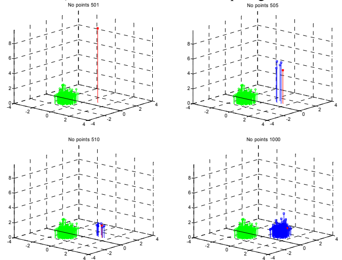
Fig. 12. The result of incremental LOF algorithm ( k=10 ) on dataset consisting of 500 records of Normal distribution N(\boldsymbol{\mu}_1, \Sigma) followed by 500 records with Normal distribution N(\boldsymbol{\mu}_2, \Sigma) . \boldsymbol{\mu}_1 = [-1 -1], \boldsymbol{\mu}_2 = [+1 +1], \Sigma = \text{diag}(0.1, 0.1) after a) n=501 ; b) n=505 ; c) n=510 ; d) n=1000 points inserted. New data records (inserted at time instant n ) are marked red.
