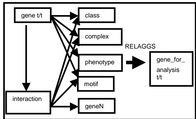
Figure 9. Propositionalization.
