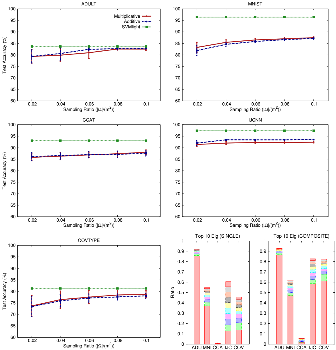
Figure 2: Prediction accuracy on test sets for 5k/5k subsets of the five UCI data sets, over different sampling ratios in kernel completion. The average and standard deviation over multiple trials with random \Omega and N = 3 nodes are shown. The bottom-right plot illustrates the proportion of the entire eigen-spectrum concentrated in the top ten eigenvalues.
