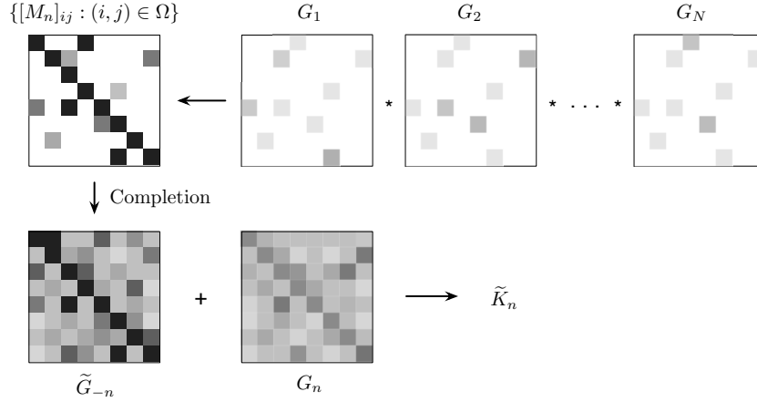
Figure 1: A schematic of kernel completion, with MULTIPLICATIVE kernel. Each node n (i) collects and summarizes the samples corresponding to \Omega from remote kernel matrices \mathbf{G}_n as the known entries of the matrix \mathbf{M}_n , and then (ii) fills up the unknown entries of \mathbf{M}_n via matrix completion, producing \tilde{\mathbf{G}}_{-n} , (iii) forming an estimate of kernel matrices together with the exact local kernel \mathbf{G}_n .
